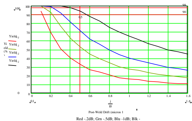
Figure 10: Yield Variation with P-WS
