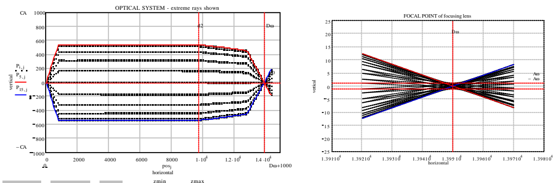
Figure 3: Ray diagrams for the first optical 'module' – showing also the result about the focal point.
