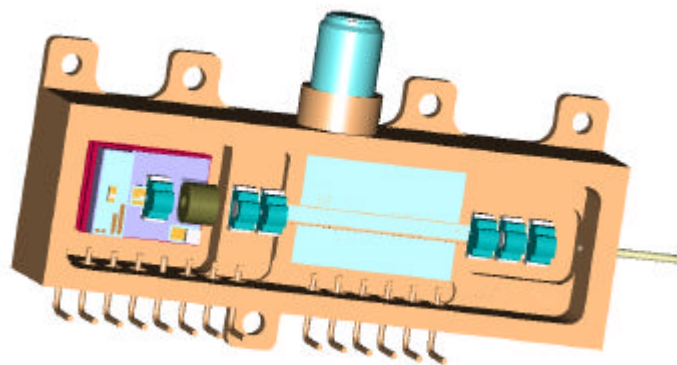
Figure 1: Pro-Engineer drawing of the fibre-optic modulator.
