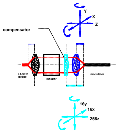
Figure 11: P-WS Compensating Lens.
