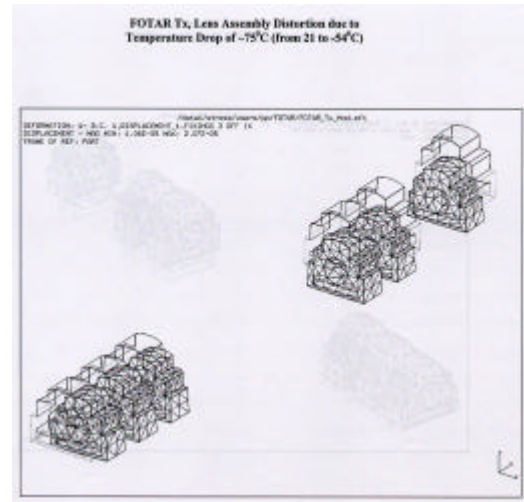
Figure 8: Movement of the Lenses.
