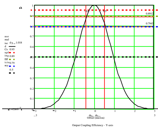
Figure 9: Coupling Variation with Vertical Position.
