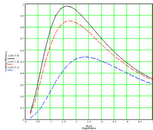
Coupling Efficiency as a Function of Magnification Showing the Effect of a One Micron Shift of the Final Lens in the X (red) - and Y (blue) - Directions
