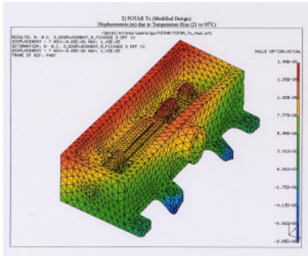
Figure 7: Typical Finite Element Model printout
