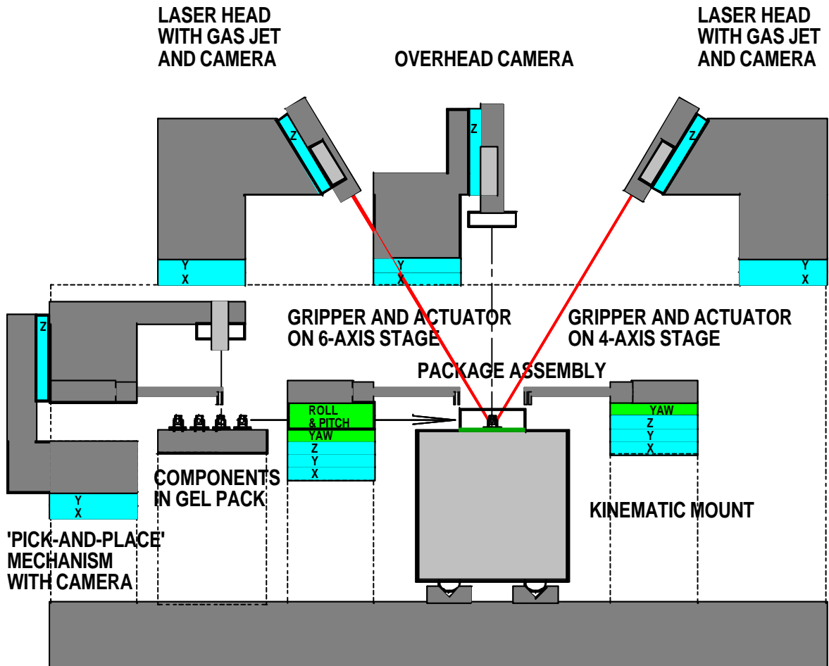
Figure 14: Principal Features of the Assembly Machine.
