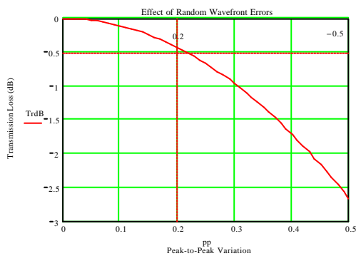
Figure 5: The effect of Wavefront Error.
