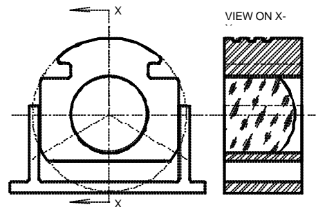
Figure 6: The lens holder and mounting clip.
