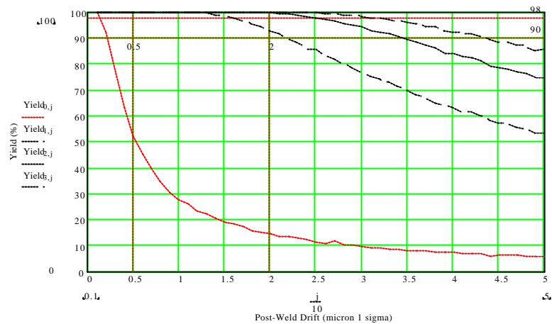
Figure 12: Yield Variation with P-WS
