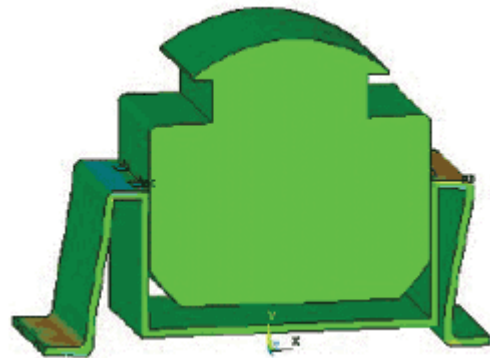
Finite element model of lens in holder and clip
